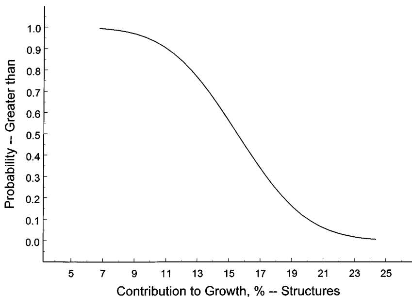
FIG. 5. Contribution to growth (structure-specific).
