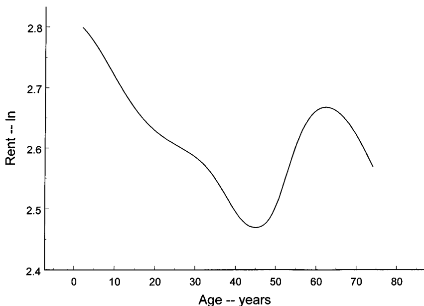
FIG. 2. Rent as a function of age.
