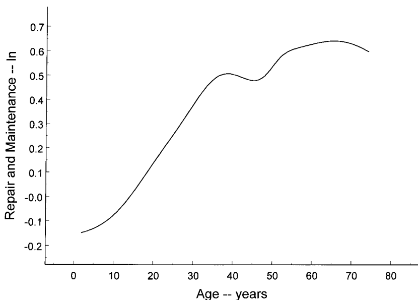
FIG. 3. Repair and maintenance as a function of age.
