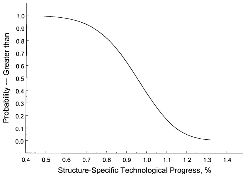
FIG. 4. Structure-specific technological progress.
